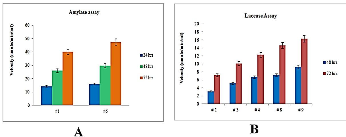
Figure 2: Assay of extracellular amylase and laccase enzymes of isolated bacterial strains. The results are represented as Mean \pm SE of three replicates.
