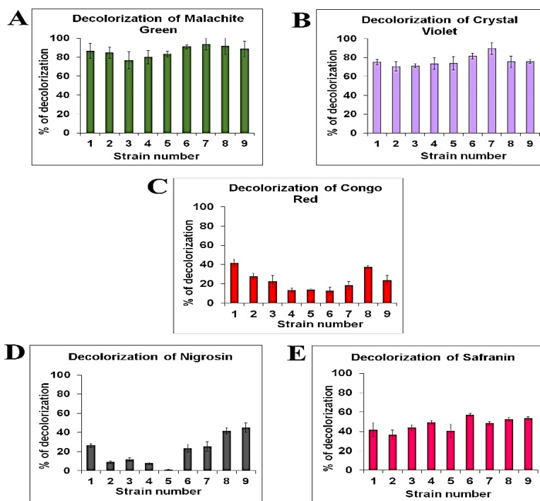
Figure 1: Dye decolourization assay of nine bacterial isolates using five different dyes namely malachite green, crystal violet, congo red, nigrosin and safranin. All the experiments were repeated thrice and the data in the graph is represented as Mean \pm SE.
